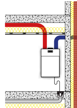
A) LEFT SET-UPS STANDARD CONFIGURATION
