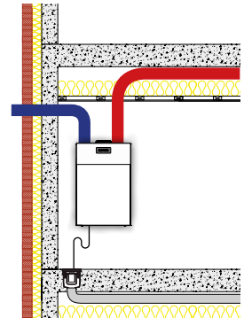
(B) RIGHT SET-UPS CAN BE CONFIGURED ON SITE
